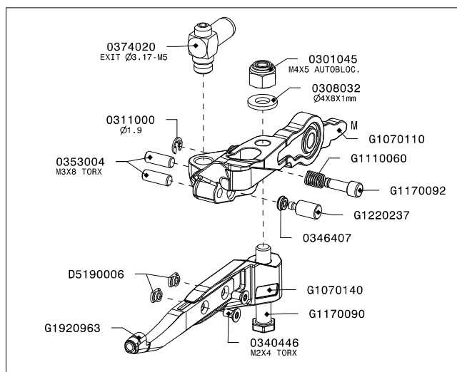
G1900636 GUIDAFILO ELASTICO MOBILE MOBILE ELASTIC YARN-FINGER
